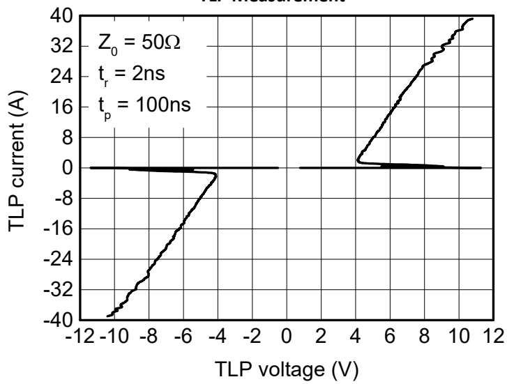
TLP Measurement
