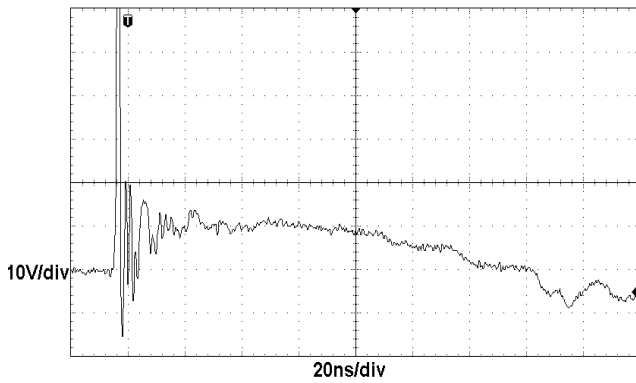
TLP Measurement
