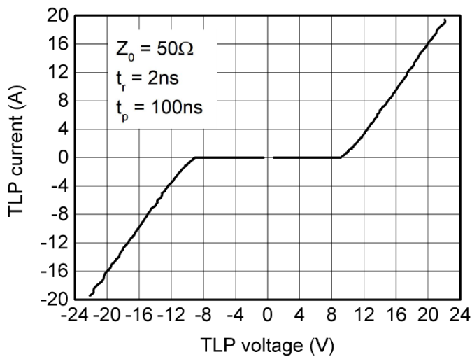
Fig.9 TLP Measurement
