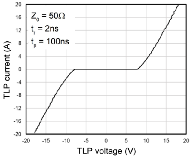
Fig.7 TLP Measurement
