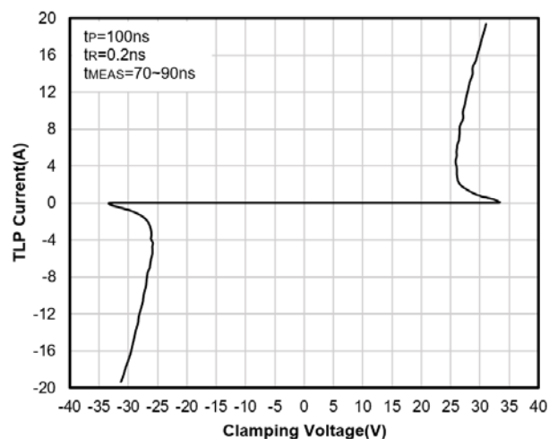
Fig.8 TLP Measurement
