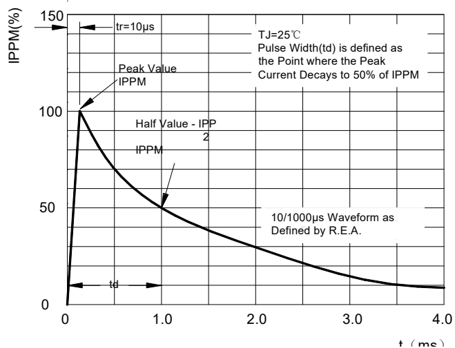
Fig1: Pulse Waveform
