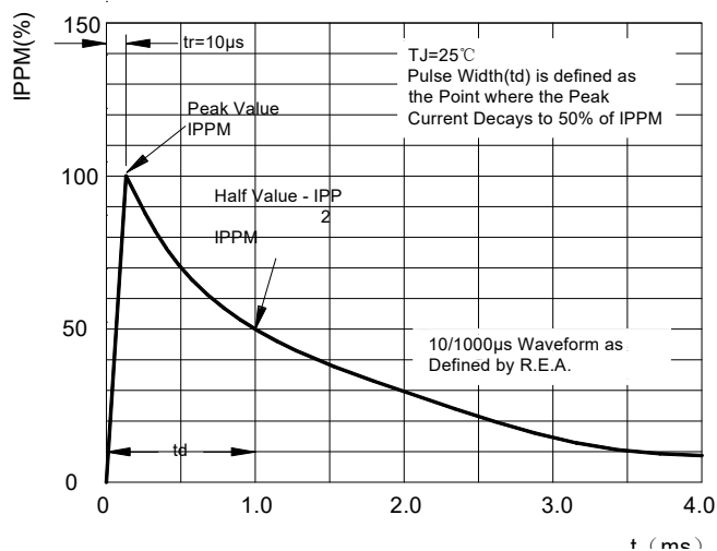
Fig1: Pulse Waveform
