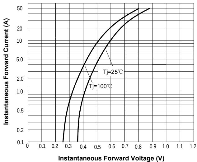
FIG3: Forward Voltage
