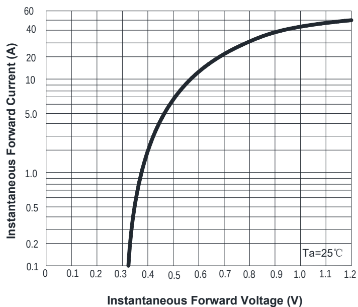
FIG3: Forward Voltage
