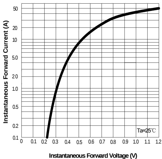
FIG3: Forward Voltage
