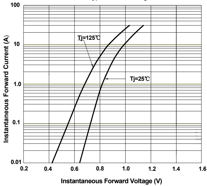
FIG.3: Typ.Forward Voltage
