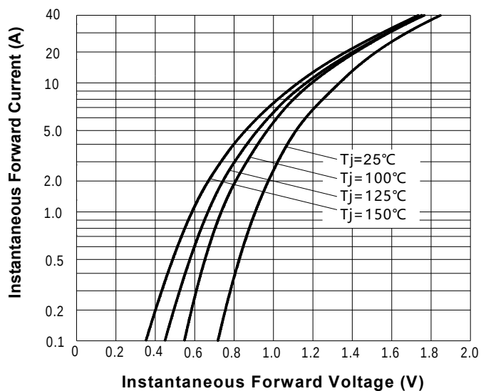
FIG3: Forward Voltage
