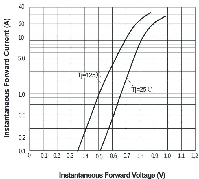
FIG3: Forward Voltage
