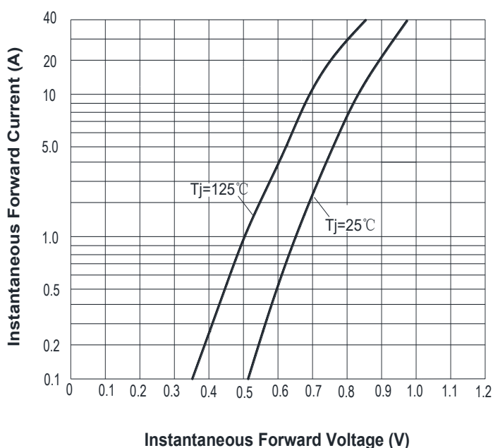
FIG3: Forward Voltage
