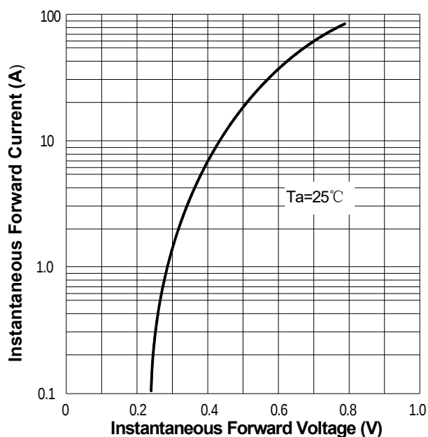
FIG.3: Forward Voltage
