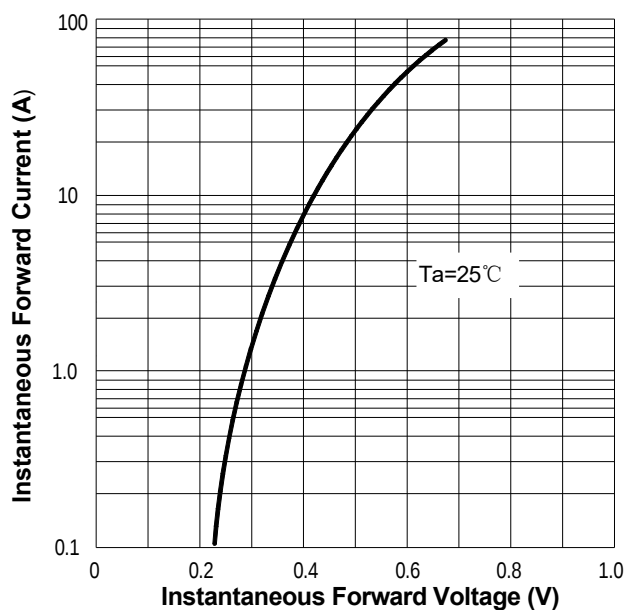
FIG.3: Forward Voltage
