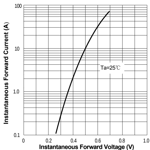
FIG.3: Forward Voltage
