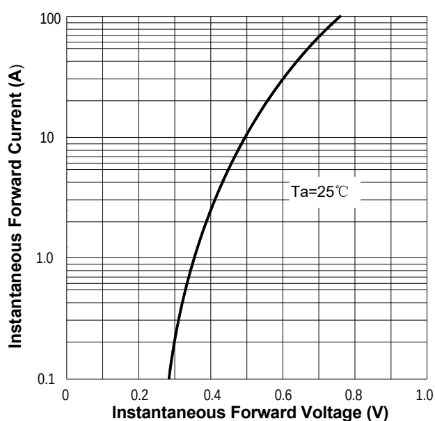
FIG.3: Forward Voltage
