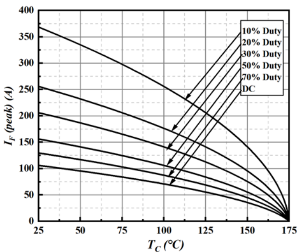
Fig7. Current Derating
