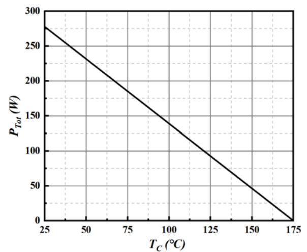
Fig6. Power Derating
