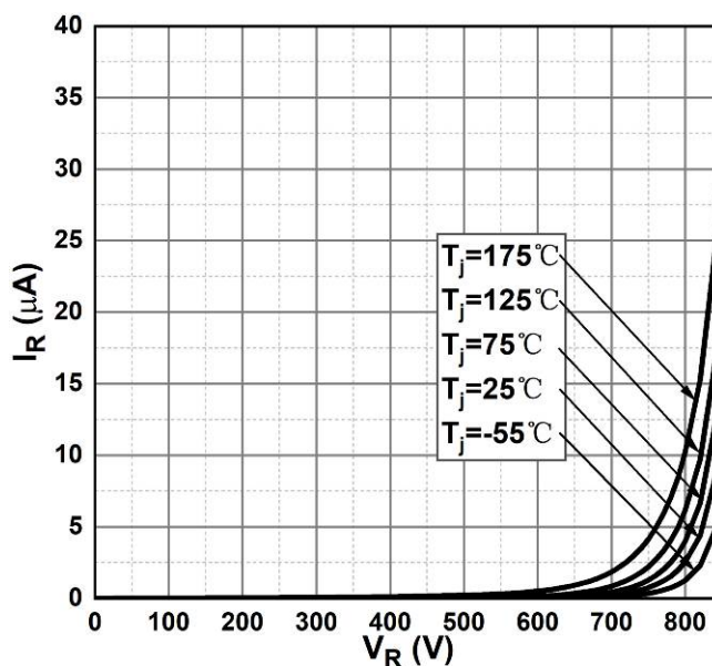
Figure 2. Reverse Characteristics
