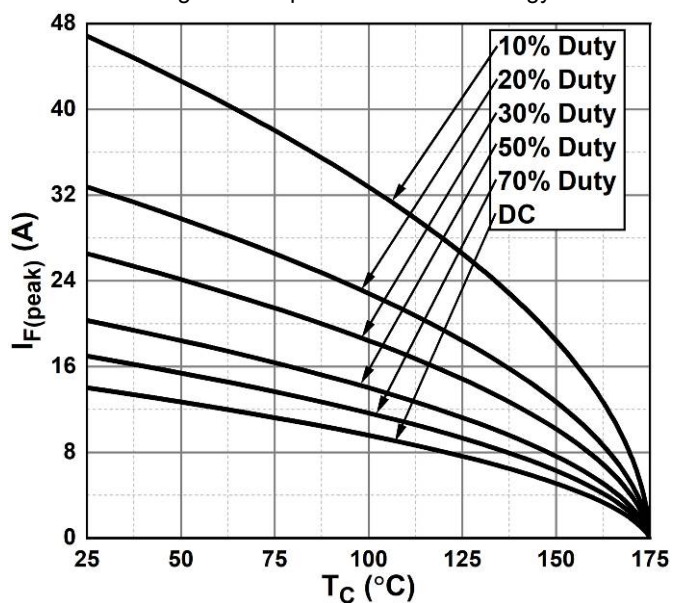
Figure 7. Current Derating
