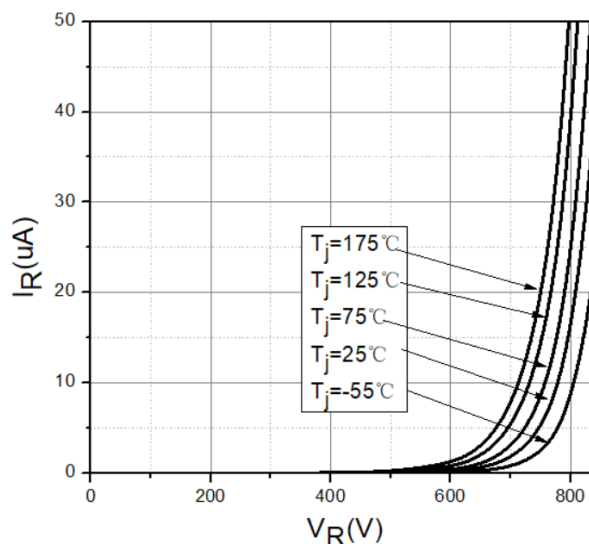
Figure2. Reverse Characteristic
