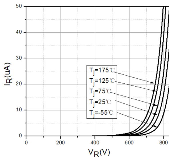
Figure2. Reverse Characteristic
