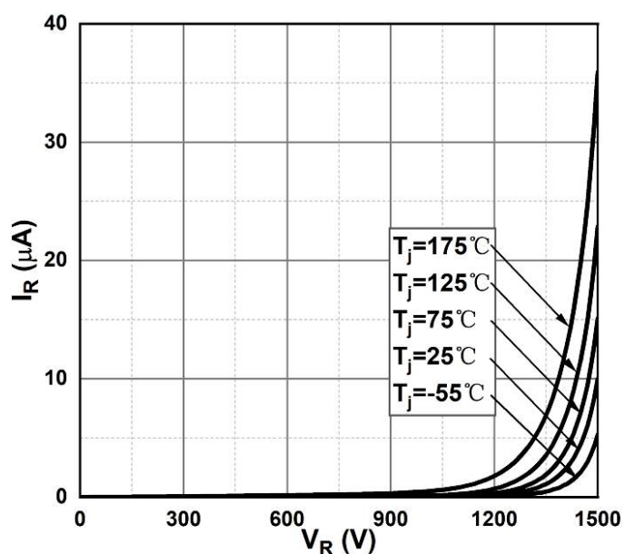
Figure 2. Reverse Characteristics
