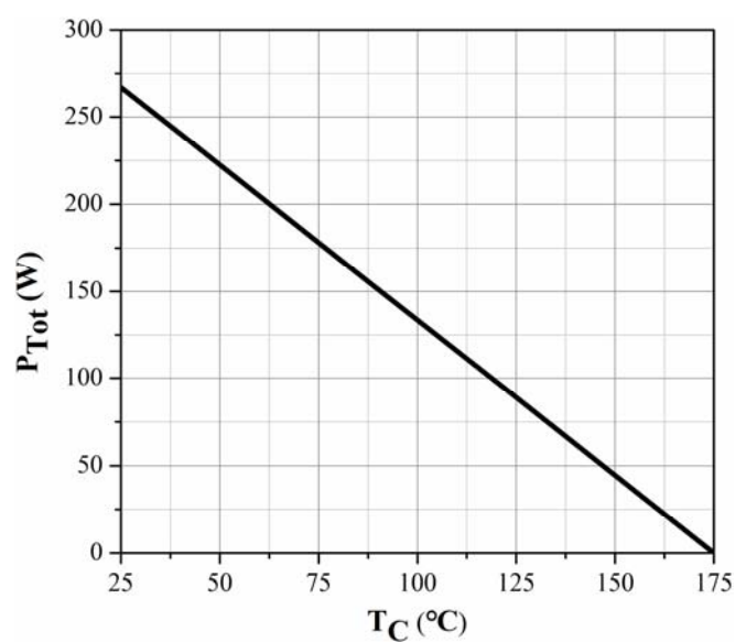
Figure 6. Power Derating
