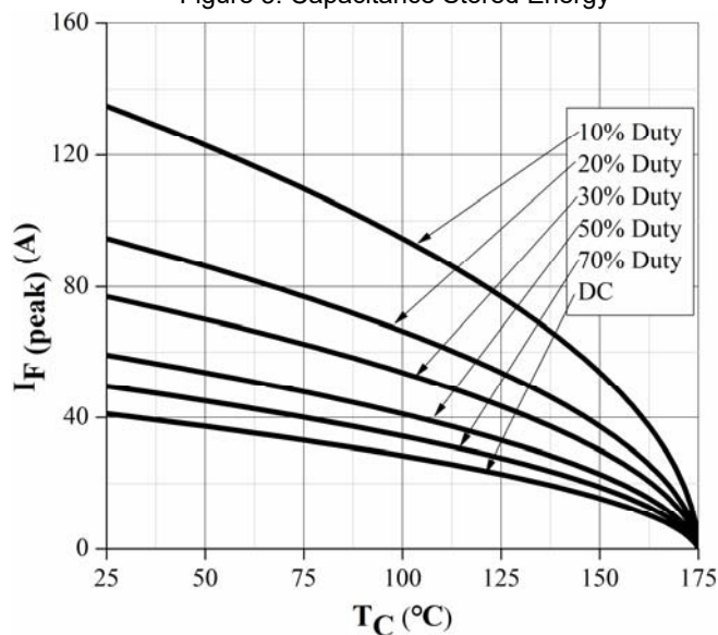
Figure 7. Current Derating
