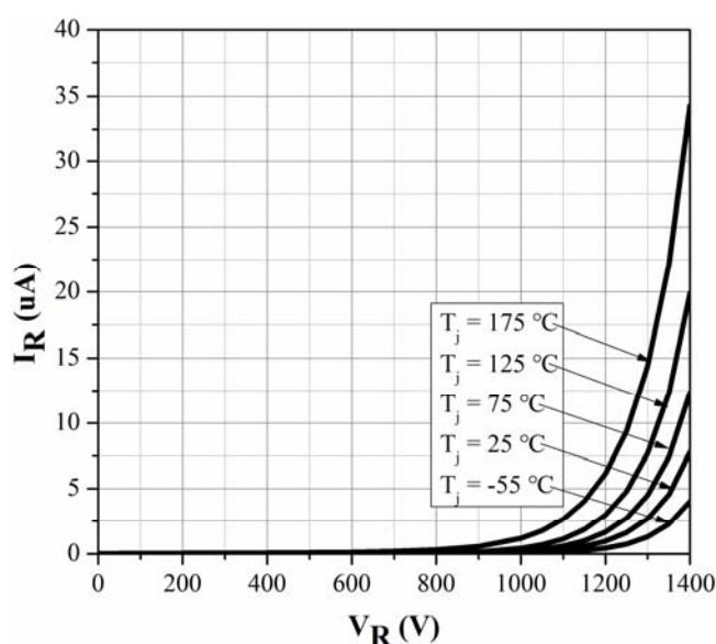
Figure2. Reverse Characteristic
