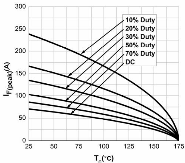
Figure 7. Current Derating
