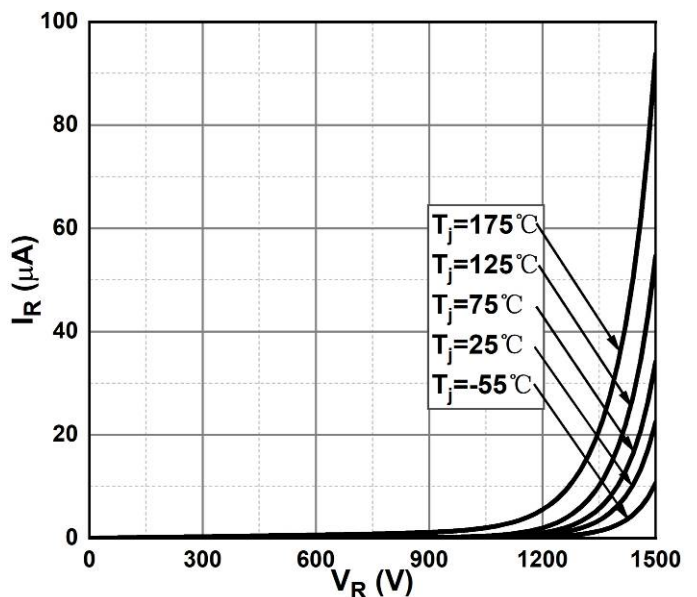
Figure 2. Reverse Characteristics
