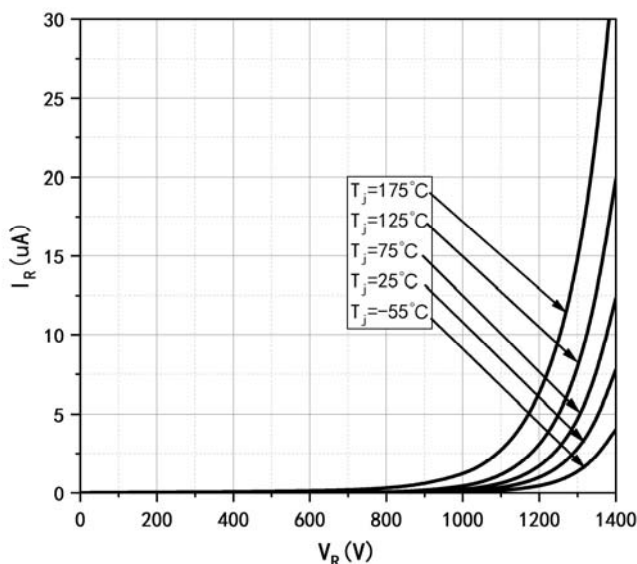
Figure 2. Reverse Characteristic
