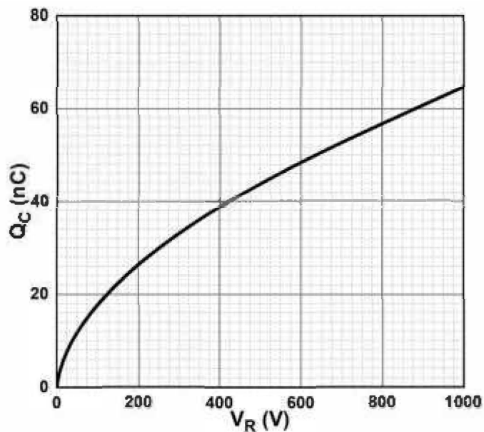
Figure 4. Total Capacitance Charge vs. Reverse
