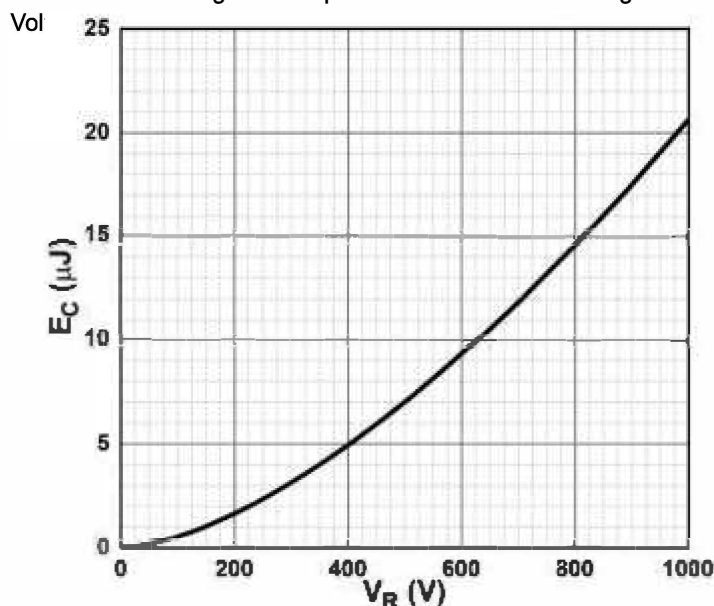
Figure 5. Capacitance Stored Energy
