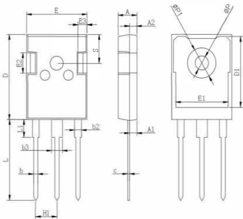
TO-247AB
