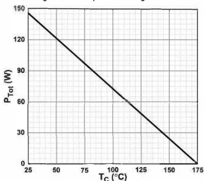
Figure 6. Power Derating
