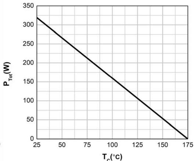
Figure 6. Power Derating
