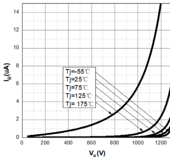
Figure2. Reverse Characteristic
