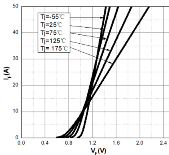
Figure 1. Forward Characteristics
