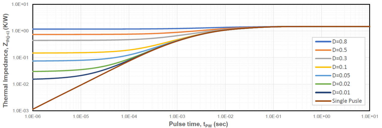
Figure 19. Transient Junction to Case Thermal Impedance
