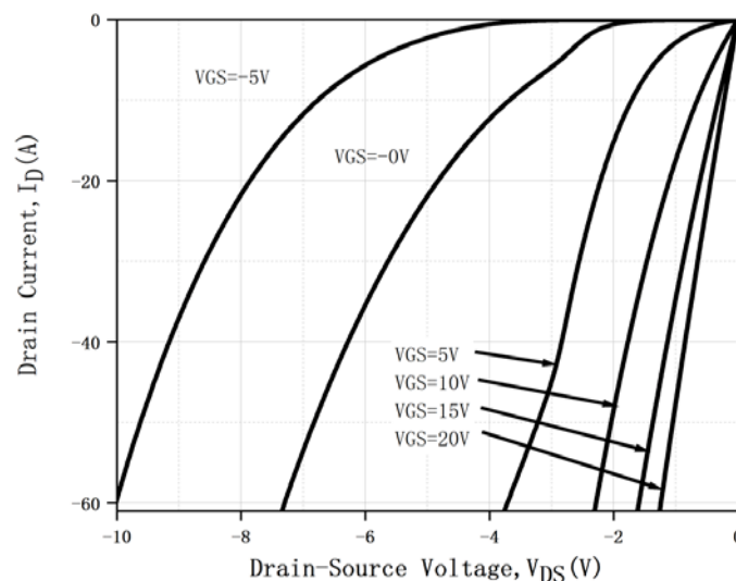
Figure 8. Reverse Output Characteristics at T_j = -55^\circ\text{C}
