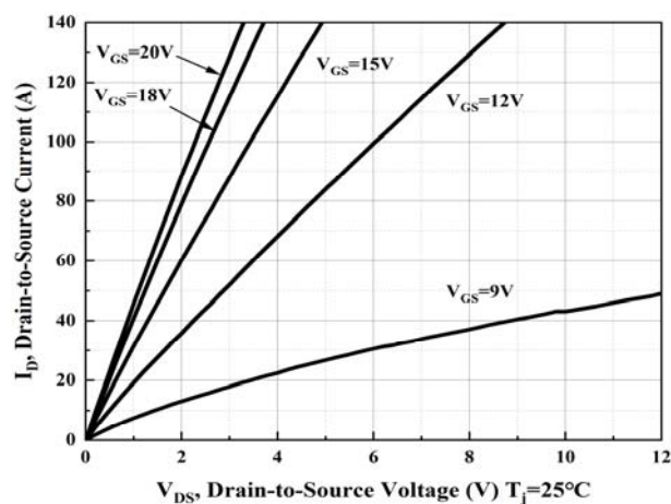
Figure2. Output Characteristics T_J = 25^{\circ}C
