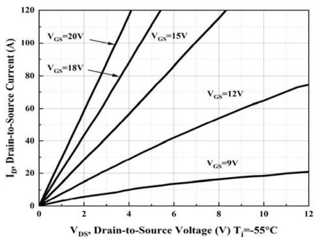
Figure 1. Output Characteristics T_J = -55^{\circ}C
