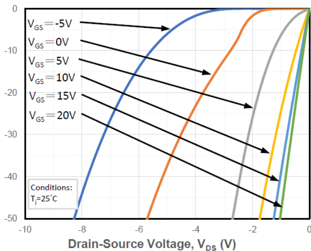
Figure 8. Reverse Output Characteristics at T_J = 25°C
