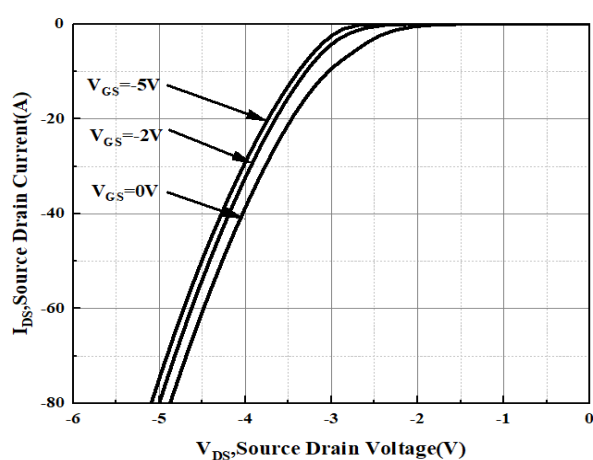
Figure 8. Body Diode Characteristic at T_j = 25^\circ\text{C}
