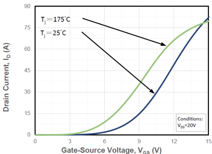
Figure 4. Transfer Characteristics for various T_J
