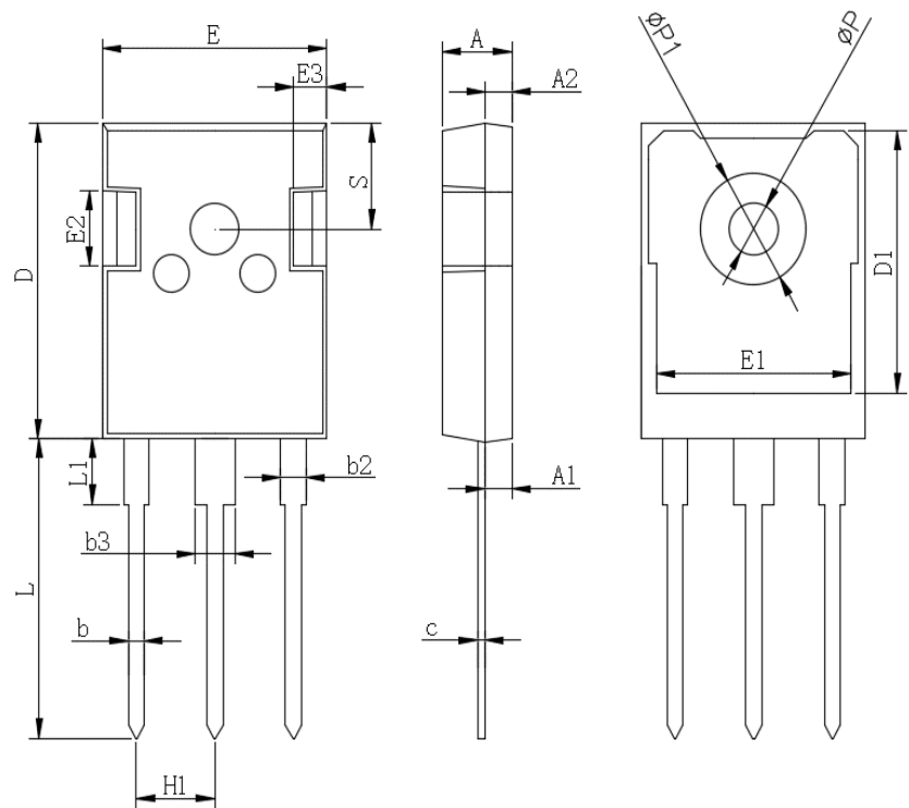
TO-247AB
