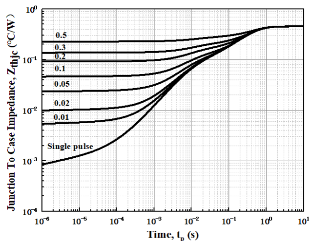
Figure 18. Transient Thermal Impedance (Junction - Case)
