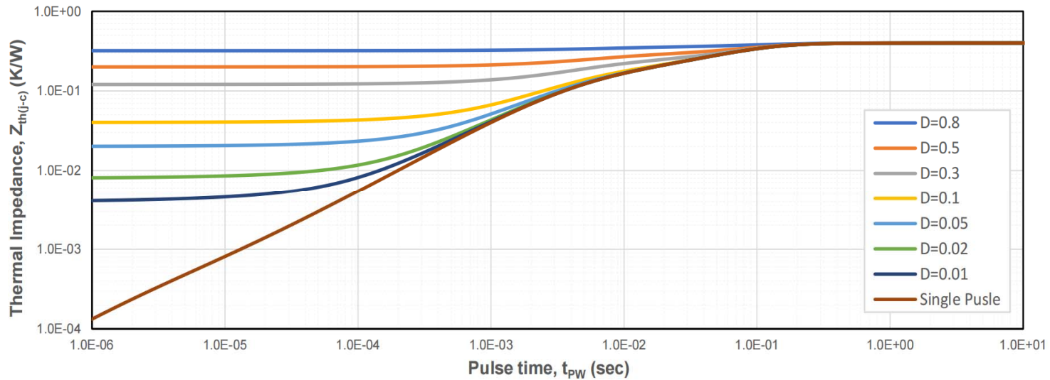
Figure 19. Transient Junction to Case Thermal Impedance
