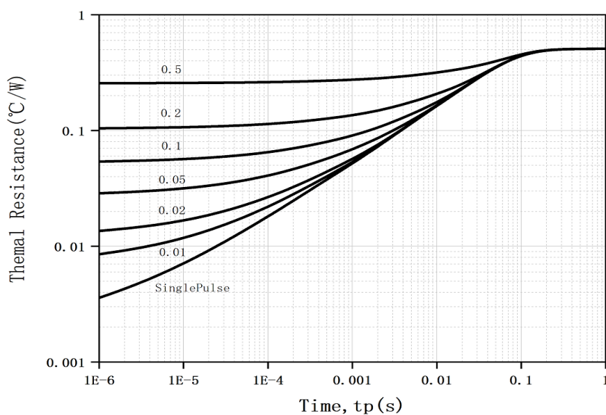
Figure 19. Transient Junction to Case Thermal Impedance
