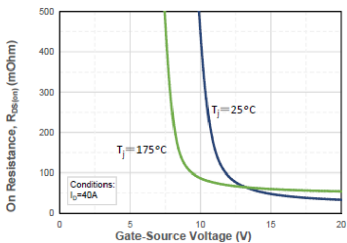
Figure 5. On-resistance vs. gate voltage for various Tj various Gate voltage
