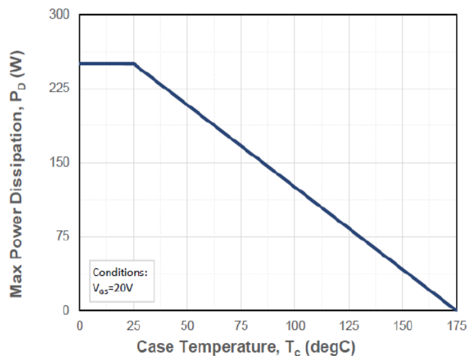
Figure 13. Maximum Power Dissipation Derating vs. Case Temperature
