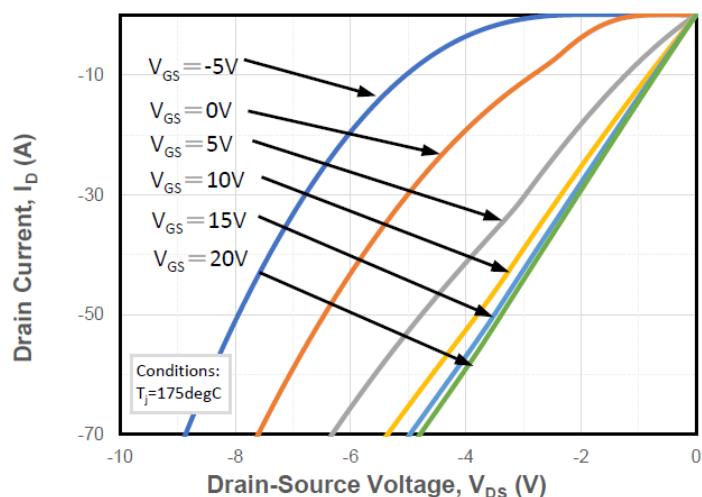
Figure 9. Reverse Output Characteristics at T_j = 175^\circ\text{C}
