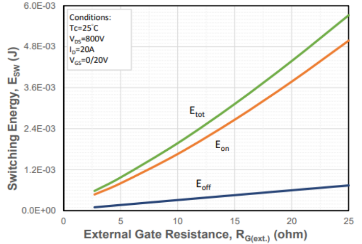
Figure 18. Clamped Inductive Switching Energy vs. External Gate Resistor ( R_{G(ext.)} )
