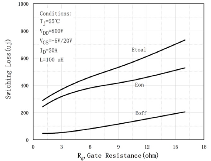
Figure 18. Clamped Inductive Switching Energy vs. External Gate Resistor ( R_{G(\text{ext.})} )
