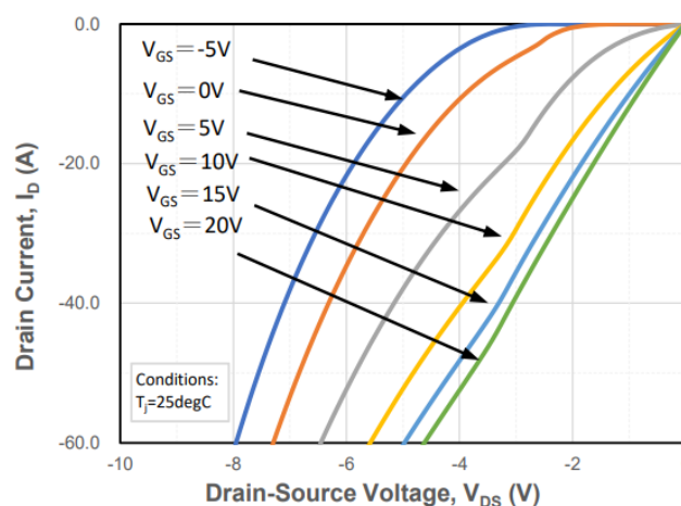
Figure 8. Reverse Output Characteristics at T_J = 25^\circ\text{C}
