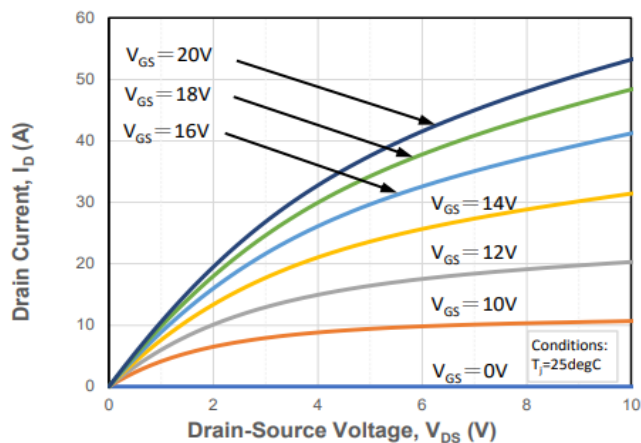
Figure 1. Output Characteristics Tj = 25℃
