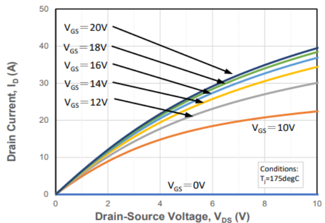
Figure2. Output Characteristics Tj = 175℃
