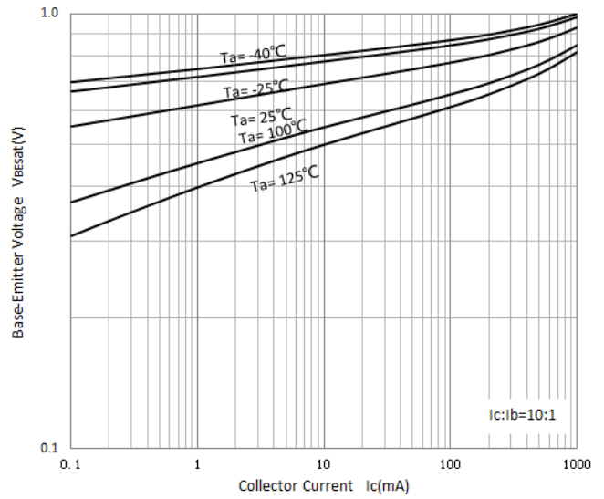
Base-Emitter Saturation Voltage
