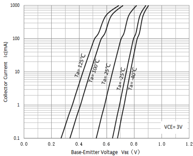
Base-Emitter On Voltage
