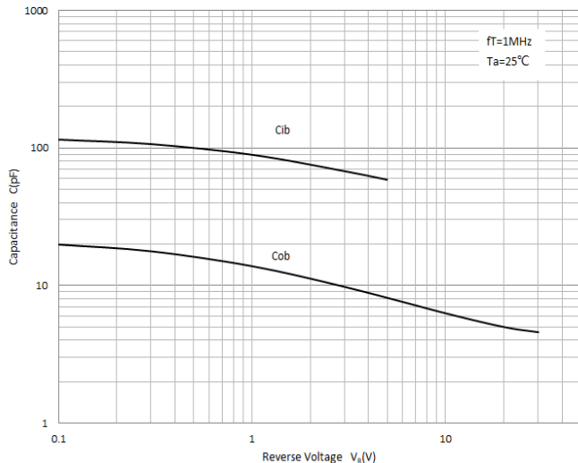
C_{ob}/C_{ib}-V_{CB}/V_{EB}
