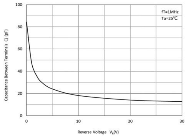
Fig 2: Capacitance Capability
