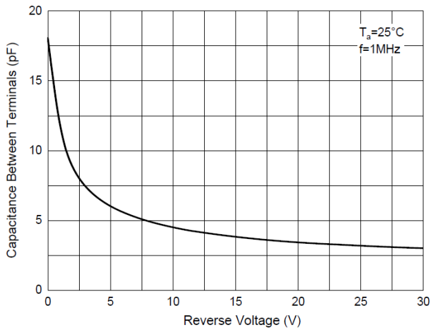
Fig. 3 - Capacitance Characteristics
